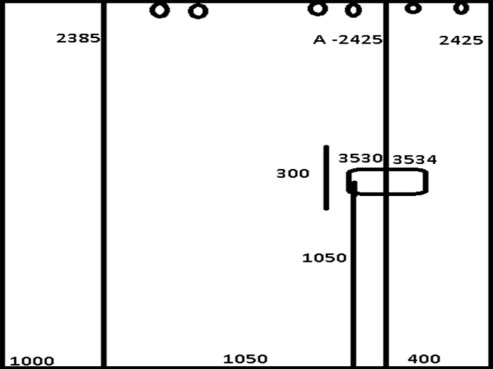
PORTA DE CORRER 8MM INCOLOR MED. 2400X2450
